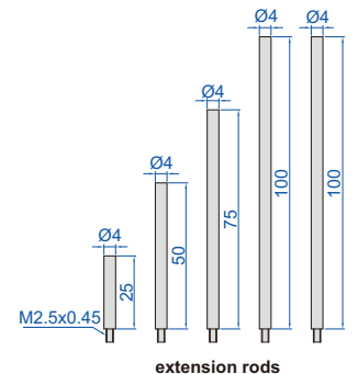
extension rods
