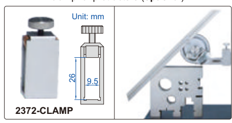
clamp for protractors (optional)
