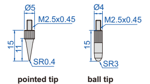
pointed tip
