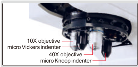
motor driven turret
