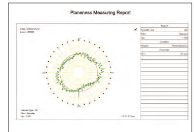
planeness analysis
