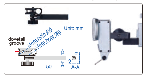
dial test indicator holder (included)
